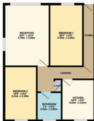
FIRST FLOOR 654 sq. ft. (260 sq. ft. approx.)
